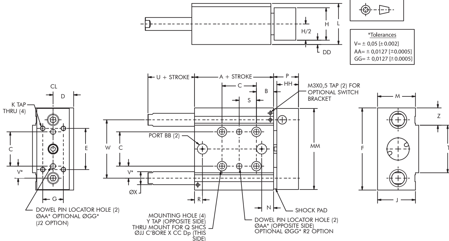
Dimensional Specifications GS Series Slide
