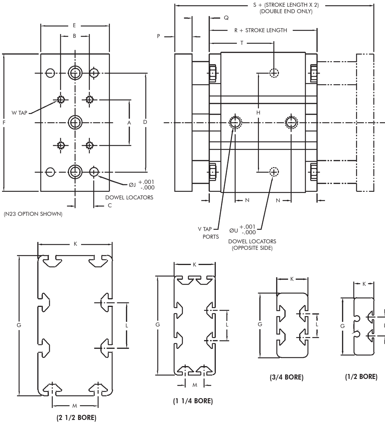
Dimensional Specifications
